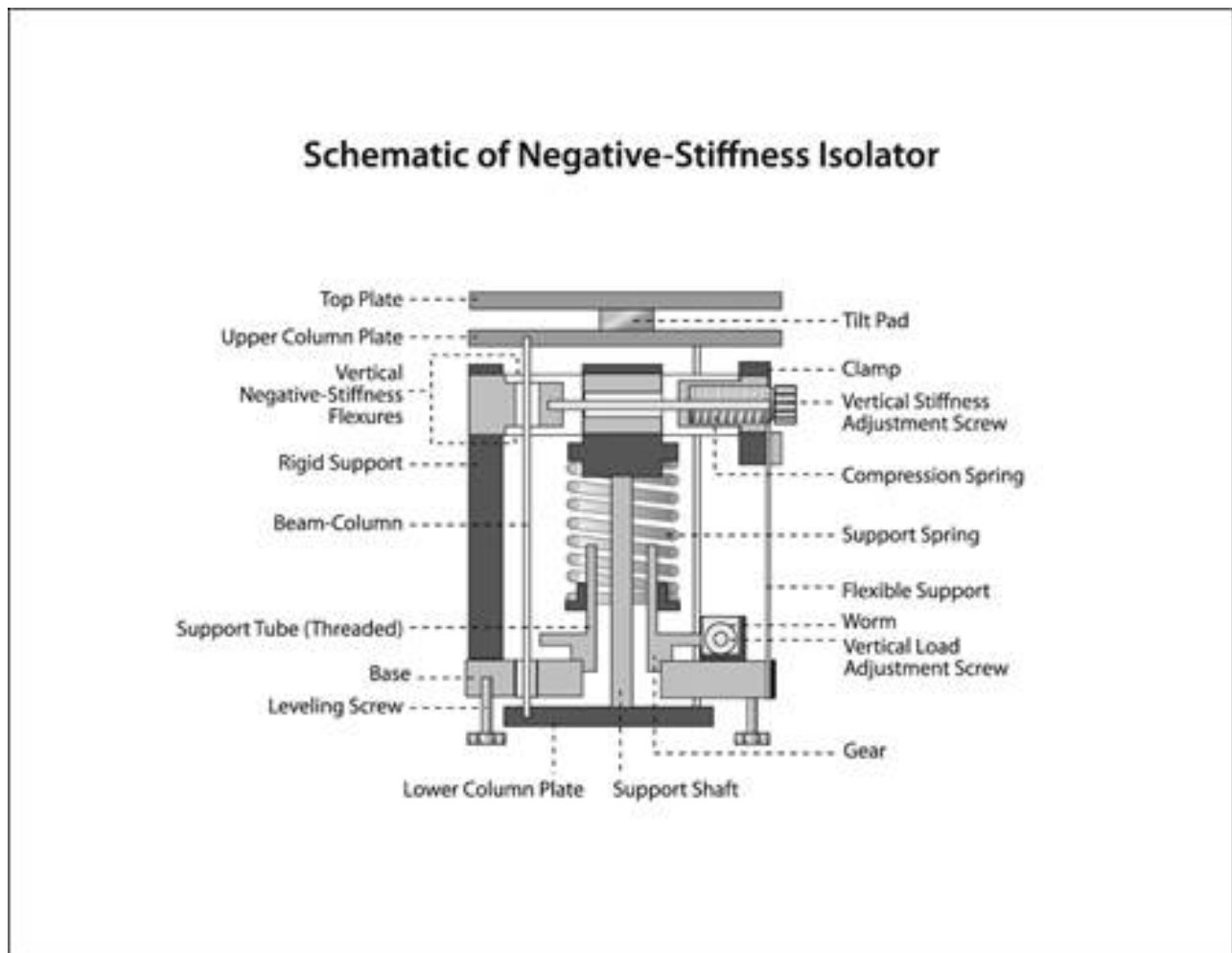
Schematic of a Minus K Negative-Stiffness Isolator
