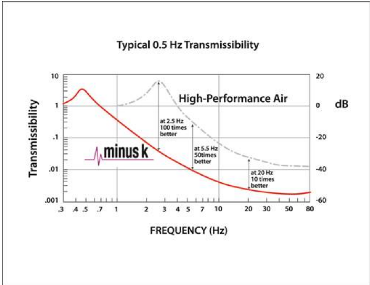
Transmissibility, Minus K Negative-Stiffness isolator versus air table.
